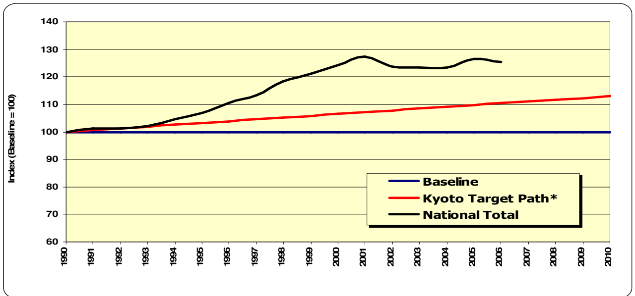
Figure 3. Index of Total GHG Emissions compared to Baseline Level and Kyoto Target Path *The straight line from baseline in 1990 to 13% above baseline in 2010 represents the Kyoto Target Path
