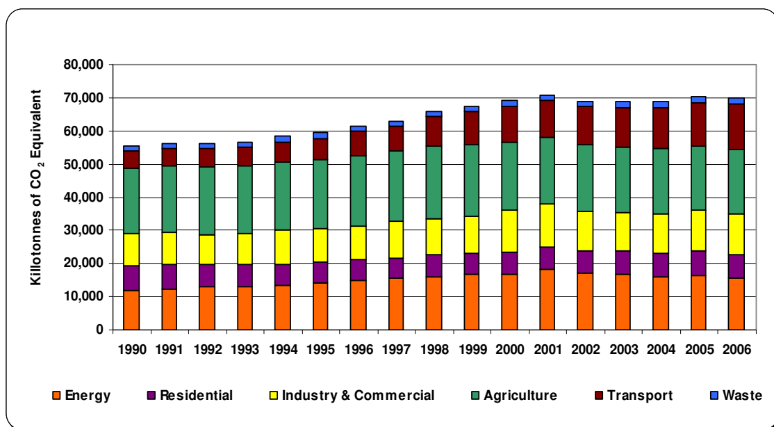
Figure 2. Trends in GHG Emissions by NCCS Sector 1990-2006
